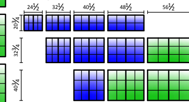
Single Glider
